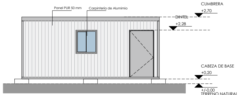
Vista Frontal
